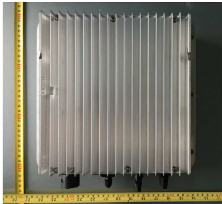
Figura 2, Vista do painel traseiro Figure 2, Rear panel view
